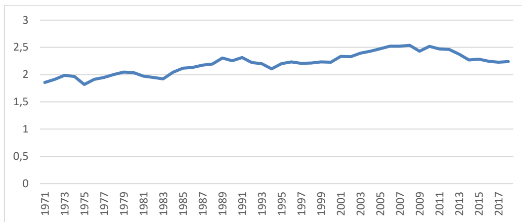
Figure 3: Univariate \sigma -convergence - Energy
